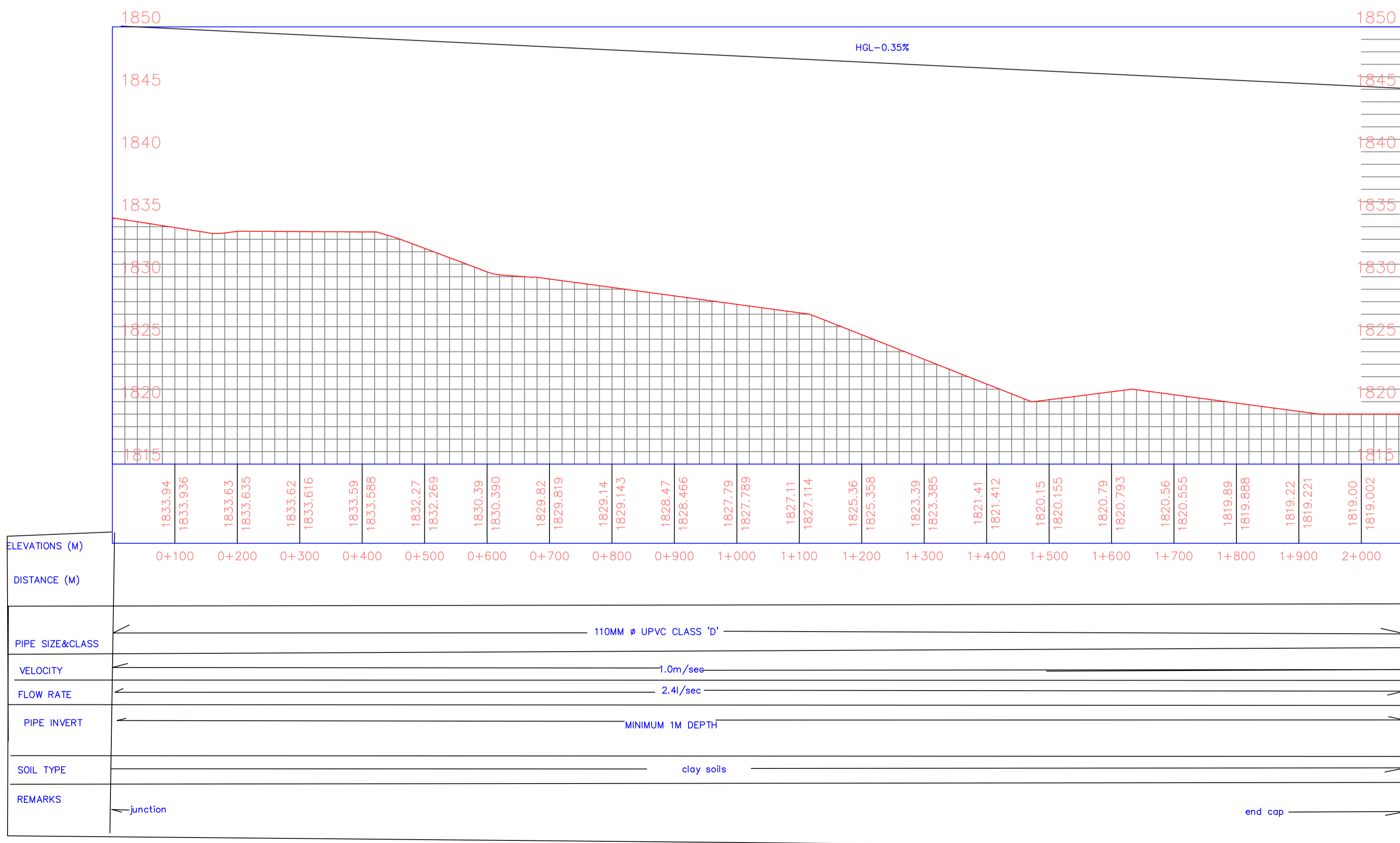
DISTRIBUTION LINE E PROFILE
